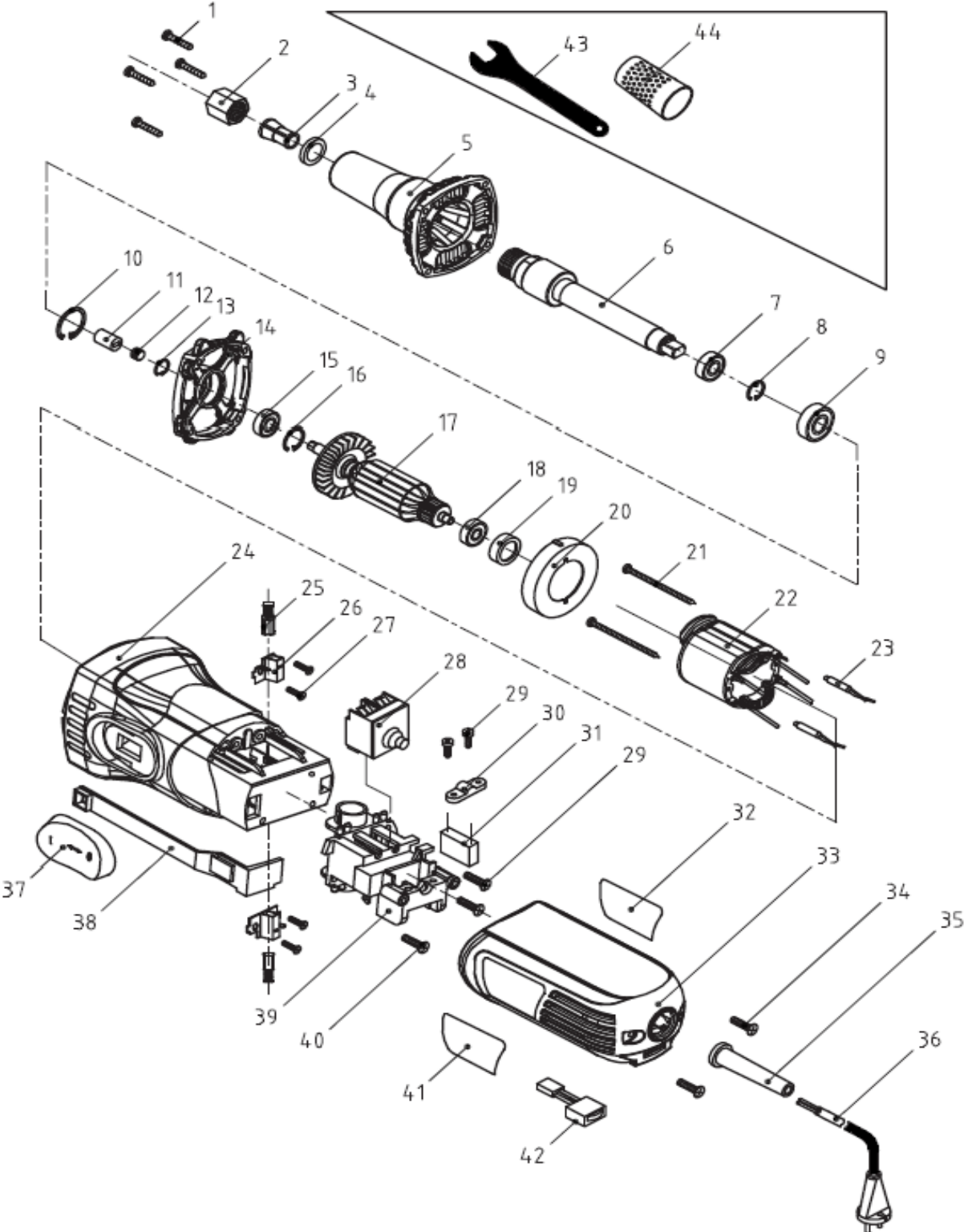
Exploded view EDG.600
